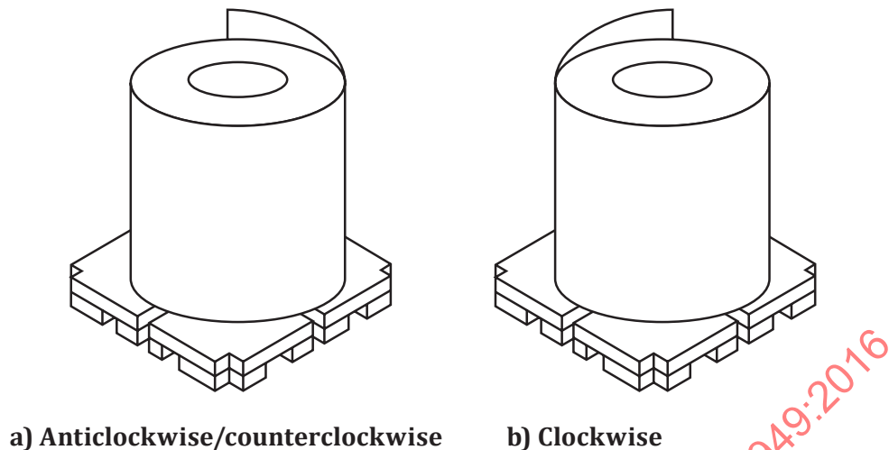
Figure 11 — Direction of coil winding
