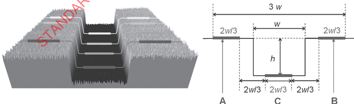
Figure 18 — Step height determination according to ISO 5436-1 (left: step height measurement standard 6 nm)
