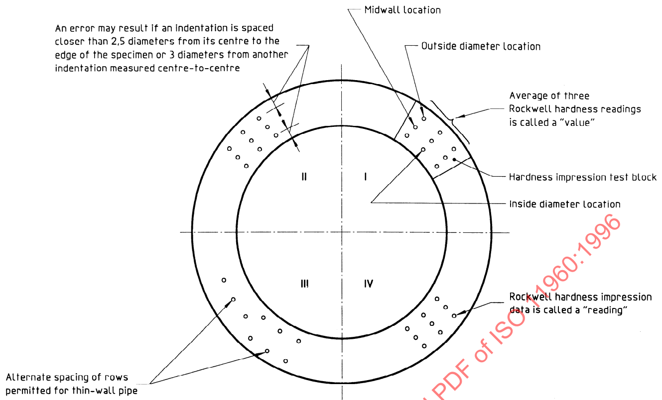
Figure 10 — Through-wall hardness test
