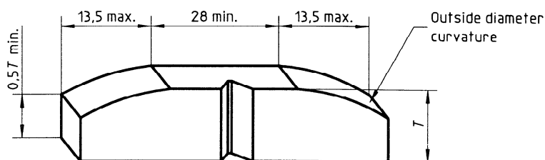
Figure 12 — Charpy specimen dimensions
