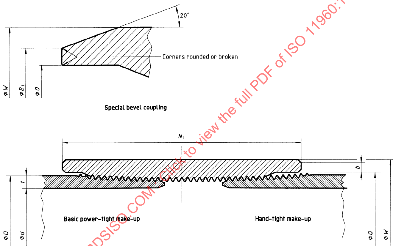
Figure 4 — Non-upset tubing and coupling
