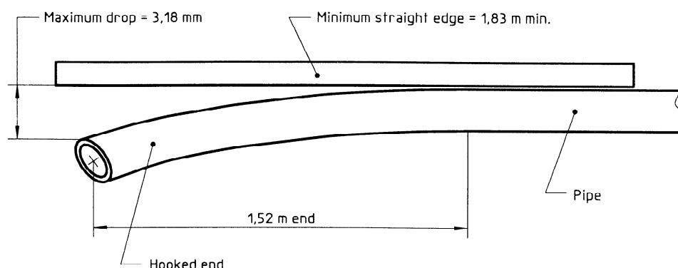
Figure 14 — Measuring end straightness
