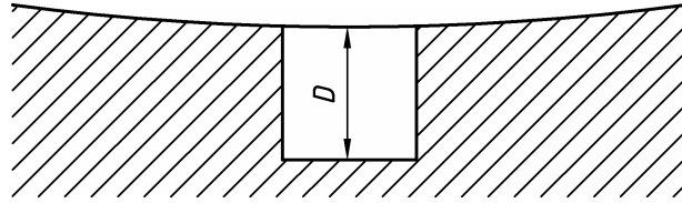
d) Flat bottomed hole
