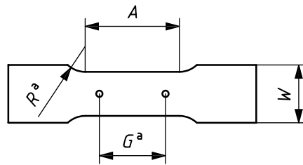
b) Strip specimen
