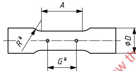
c) Round-bar specimen
