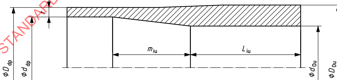
d) Internal-external upset (IEU)
