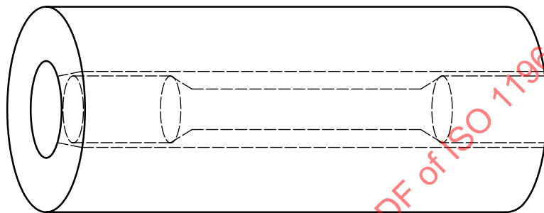
b) Drill-pipe-body tensile — Round-bar specimen
