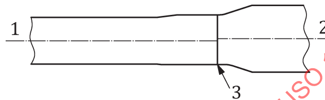
a) Upset misalignment
