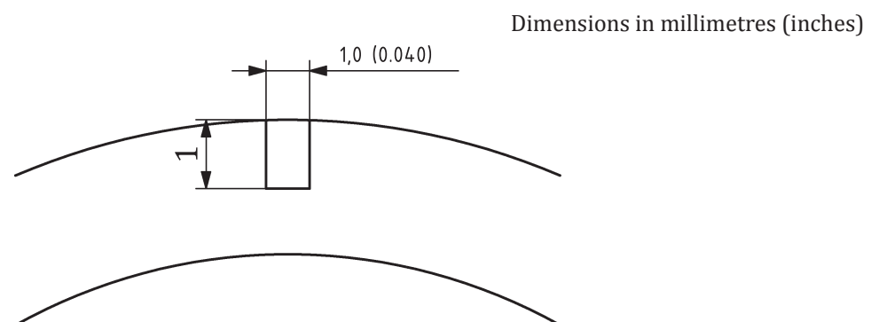
Figure B.10 — Upset and tool-joint alignment
