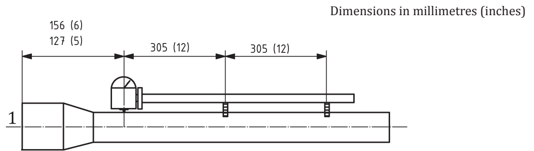
a) Upset misalignment
