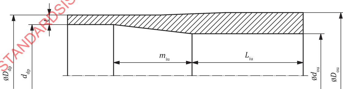
c) External upset (EU) — Grades X, G, S and E: label 1:3-1/2, label 2:13.30
