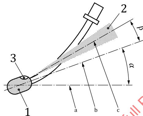
a) horizontal alignment: \alpha between 0^\circ and 5^\circ ; \beta = 10^\circ
