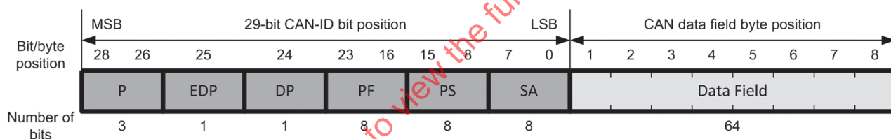
Figure 1 — PDU1 and PDU2 structure
