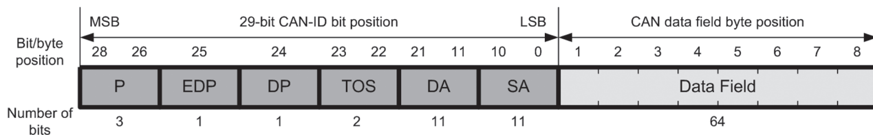
Figure 2 — PDU3 structure
