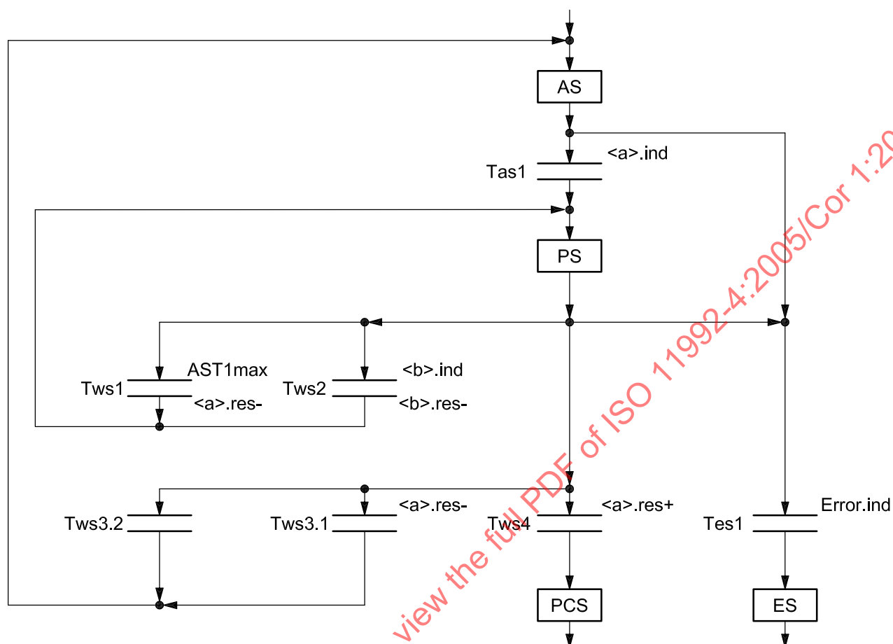
Figure 3 — Client service state diagram — Service request with physical server target address
