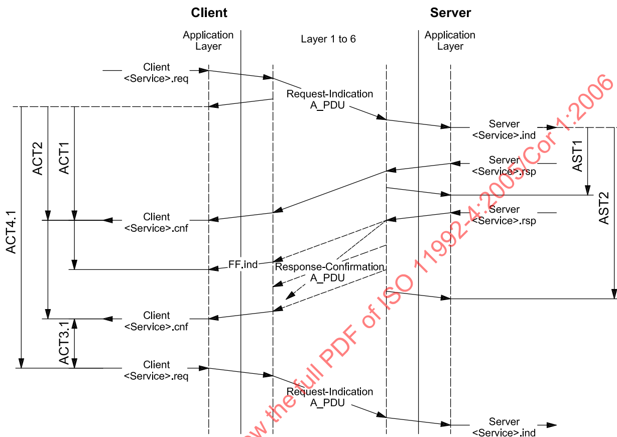
Figure 5 — A_PDU timing diagram confirmed services — physical target address
