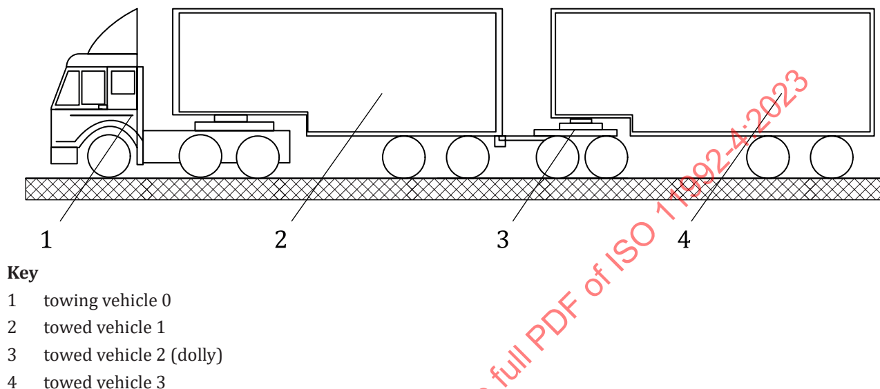
Figure 2 — Example of a possible road train configuration
