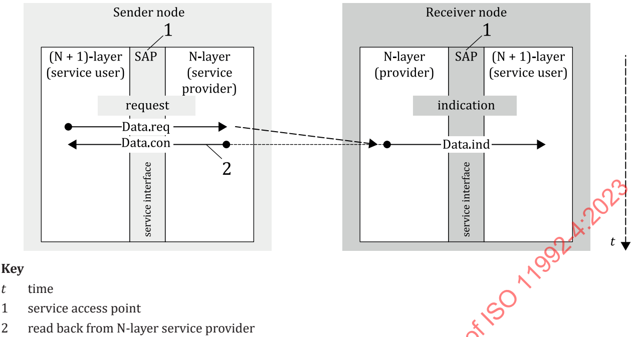
Figure 4 — A_Data.req, A_Data.ind, and A_Data.con service interface
