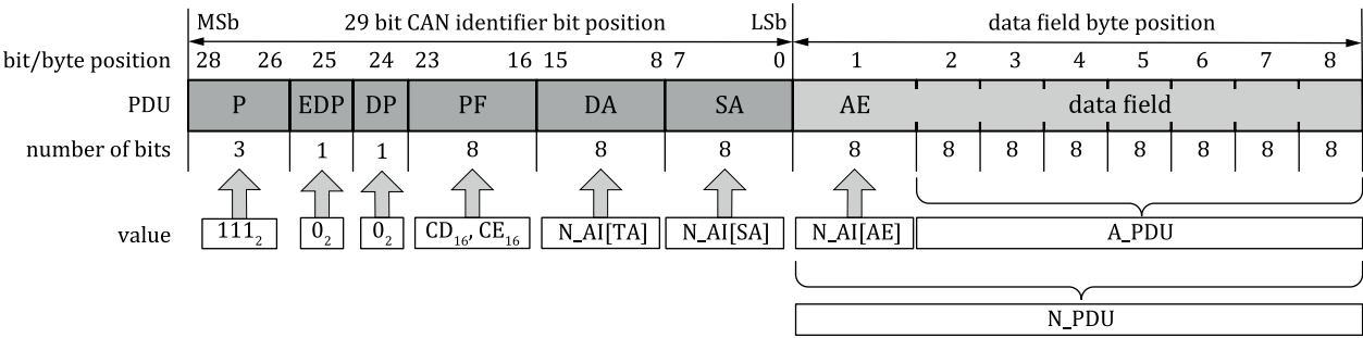
Figure 5 — Diagnostic CAN identifier configuration
