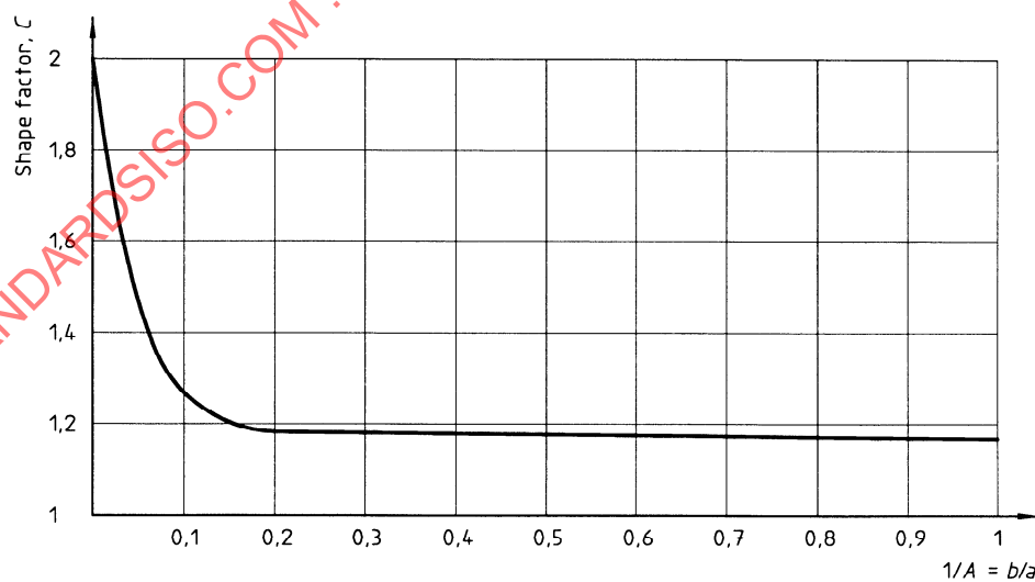
Figure 2 — Variation of "shape factor" with aspect ratio for rectangular plates perpendicular to the flow
