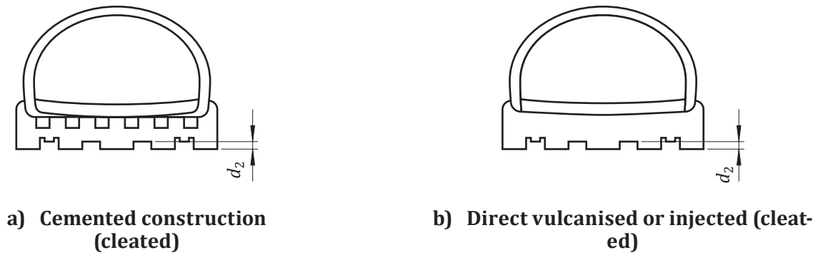
Figure 2 — Cleat height of direct injected, vulcanised and cemented outsole
