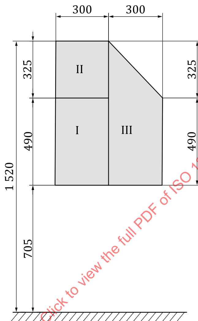
Figure B.2 — side view of accessible zone
