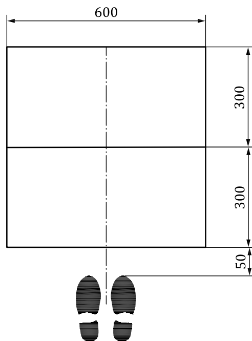
Figure B.3 — Top view of accessible zones
