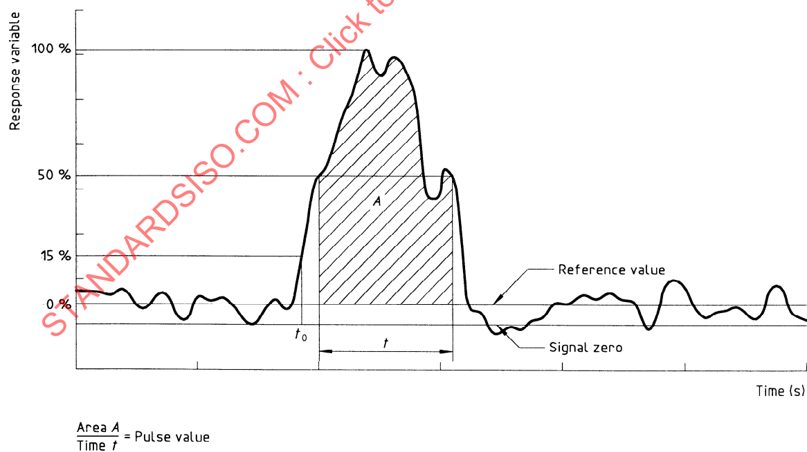
Figure 3 — Definition of pulse value (a response variable)
