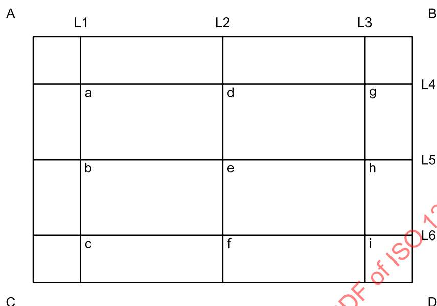
Figure 3 — Distribution of nine detection spots (top view of strips case)
