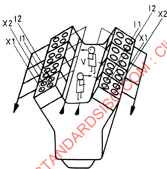
c) Inlet valves near to observer, exhaust valves away from observer, valves side-by side, exhaust manifold outside, intake manifold inside V-engine
