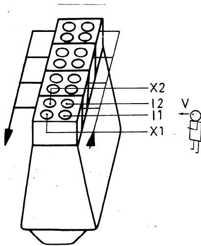
a) Inlet valves near to observer, exhaust valves away from observer, valves side-by-side, in-line engine
