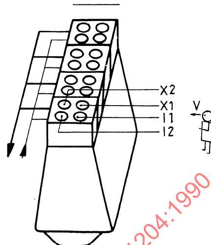
b) Exhaust valves at right, inlet valves at left of observer, valves in row, in-line engine
