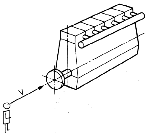
a) Right-hand single-bank engine
