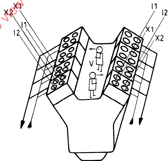
d) Exhaust valves at right, inlet valves at left of observer, valves in row, exhaust and intake manifold outside V-engine
