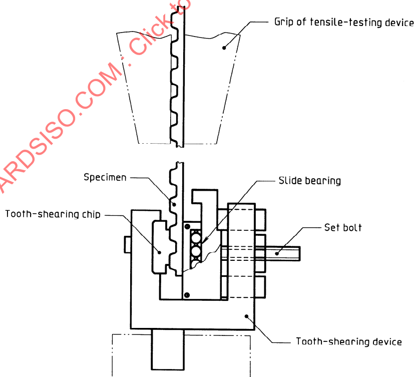
Figure 4 — Tooth-shearing apparatus and specimen
