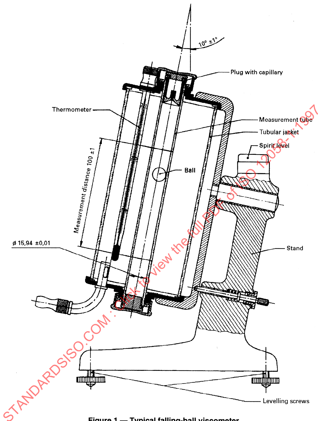
Figure 1 — Typical falling-ball viscometer
