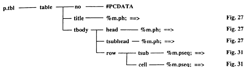
Figure A.22 Table matter elements (%p.tbl;)
