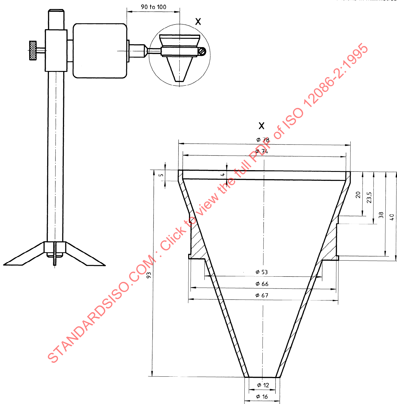
Figure 11 — Funnel for determination of flow time
