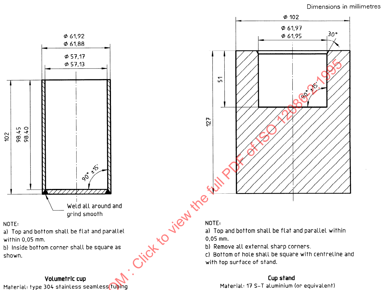
Figure 7 — Volumetric cup and cup stand for determination of bulk density
