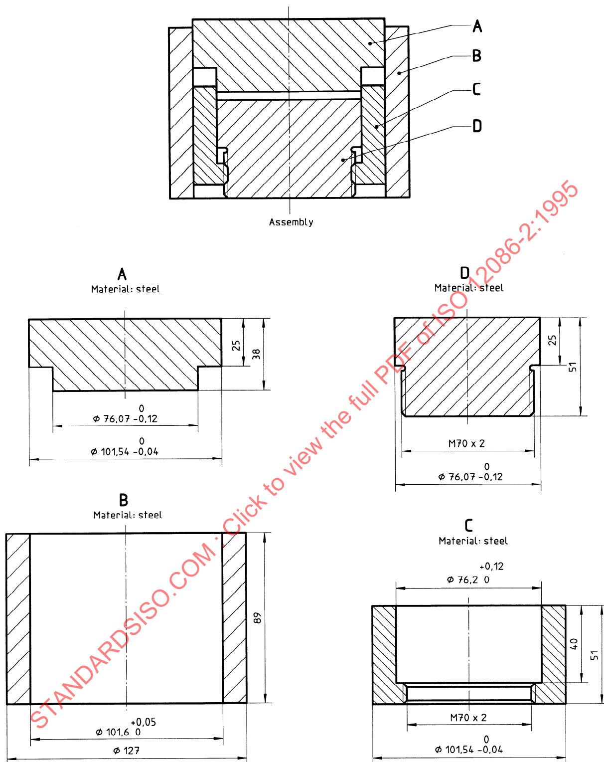
Figure 4 — Mould assembly for preparation of specimens for the determination of tensile properties
