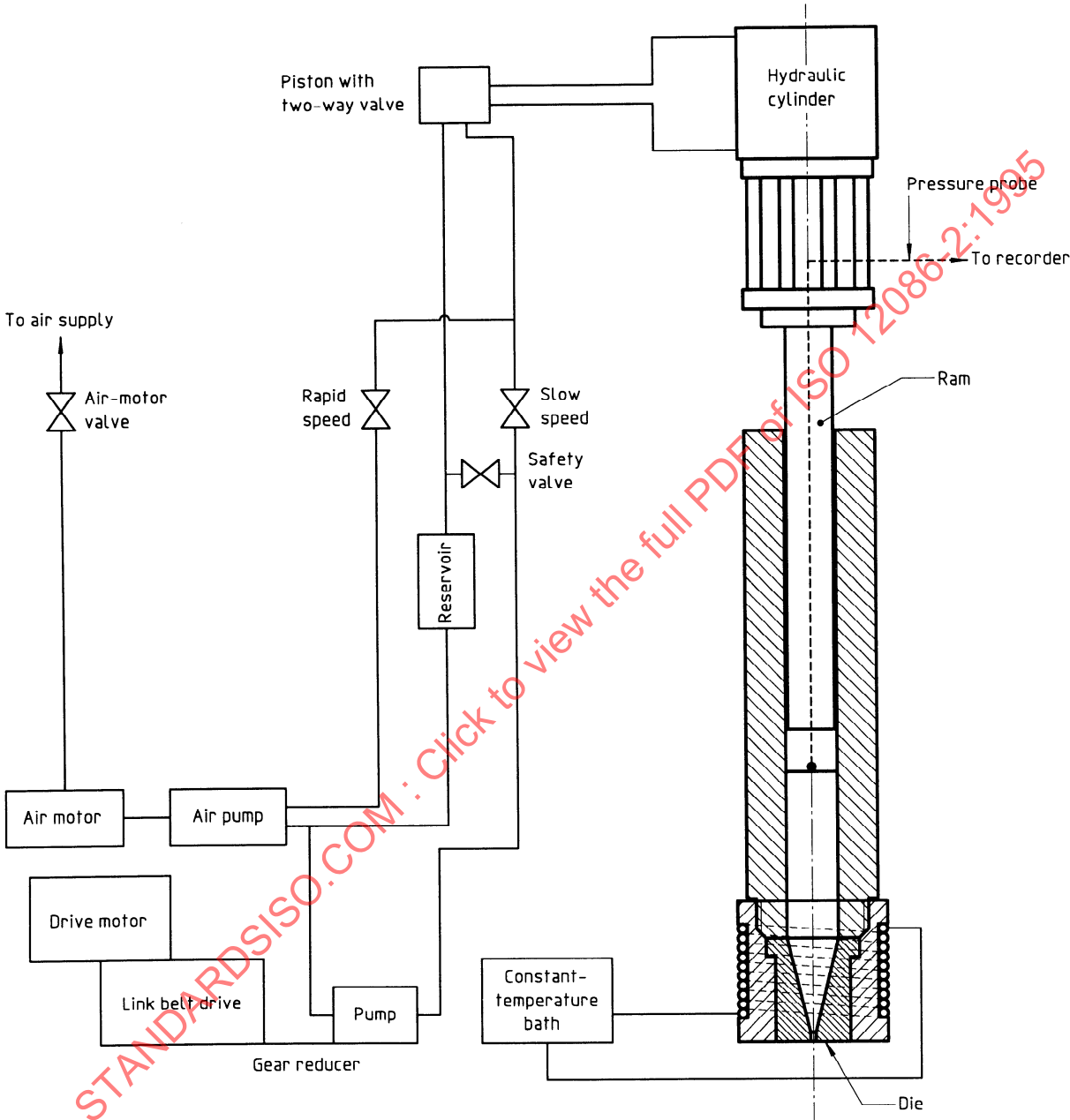
Figure 9 — Paste extruder for determining extrusion pressure
