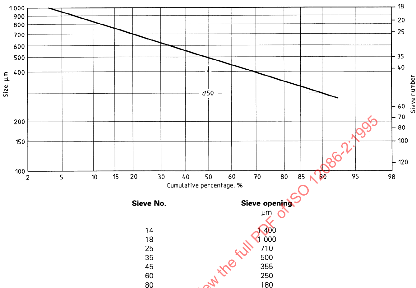
Figure 3 — Typical log/log probability plot for sieve analysis
