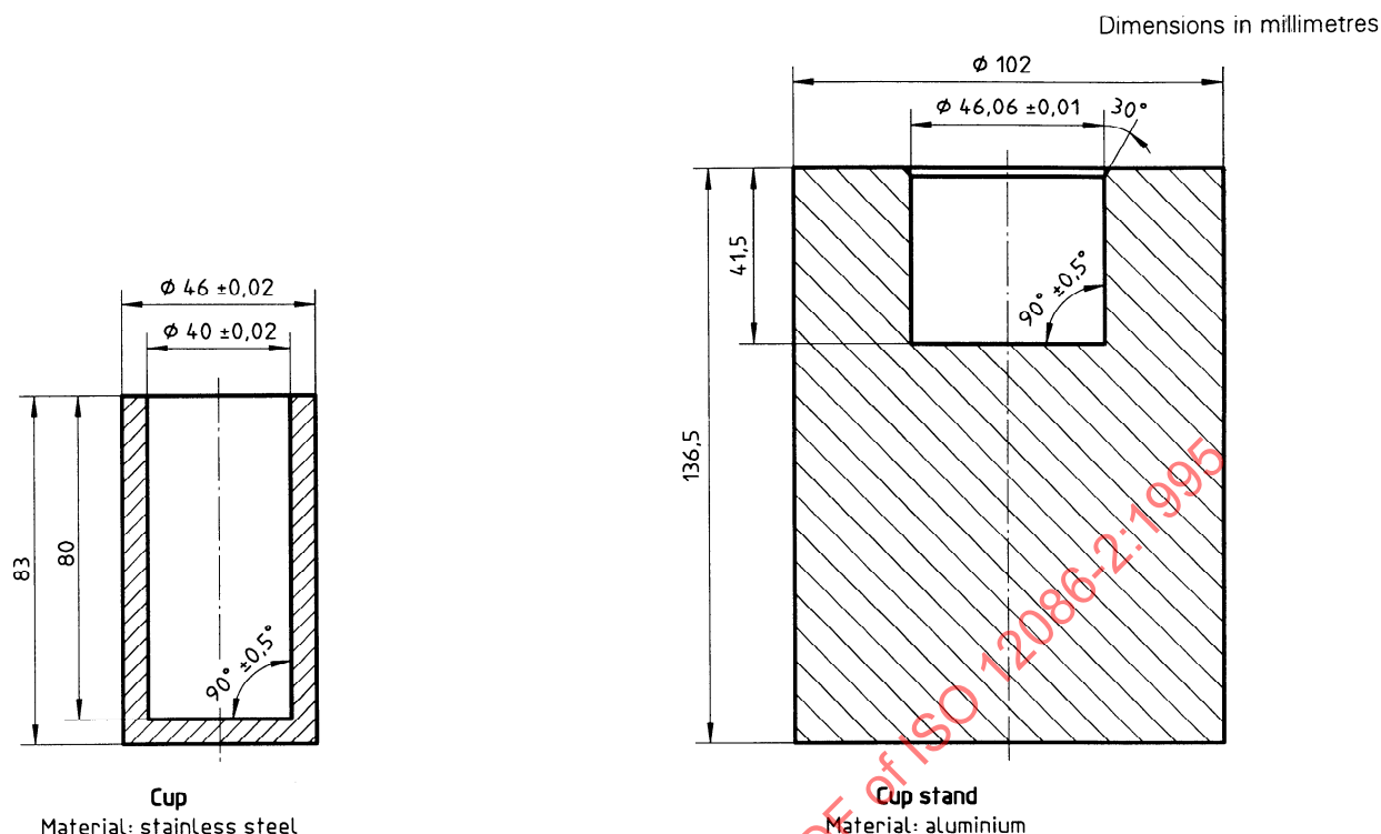
Figure 12 — Volumetric cup and stand for determination of flow time
