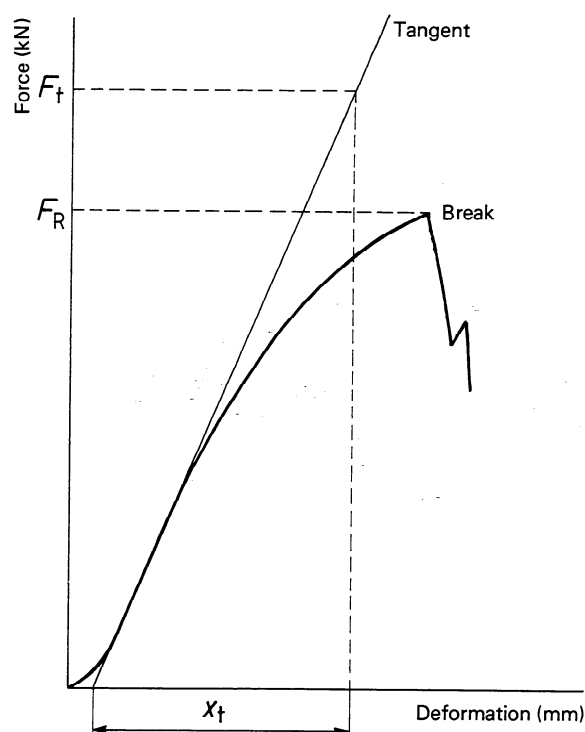
Figure 2 — Typical force/deformation diagram
