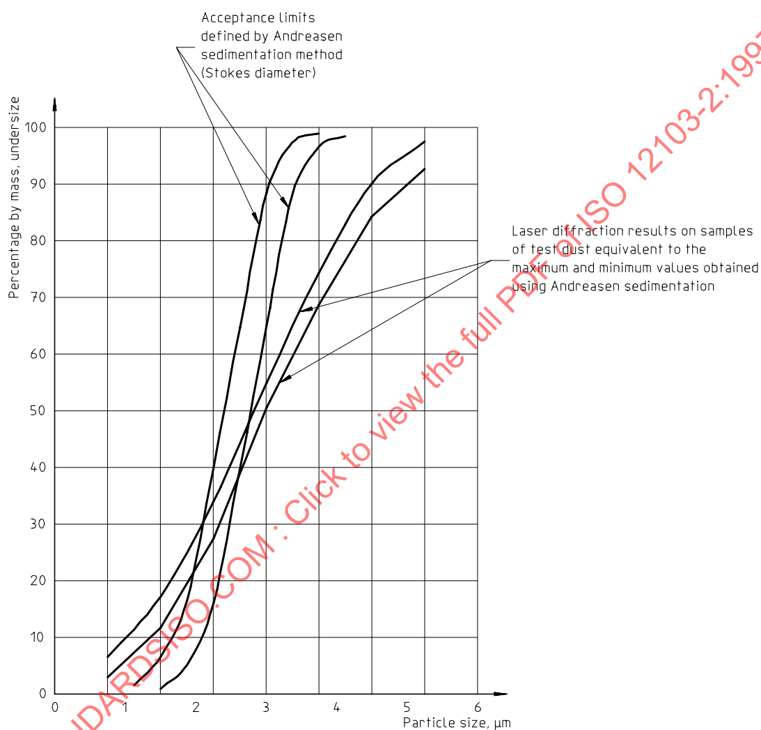
Figure A.1 — Comparison of particle size distribution using laser diffraction of ISO 12103-M2 test dust with Andreasen sedimentation
