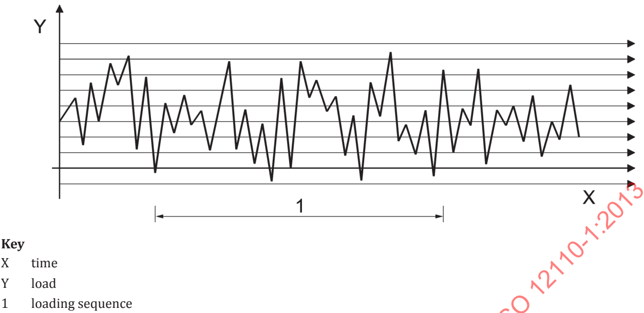
Figure 2 — Load versus time history
