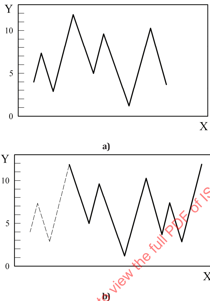
Figure A.6 — Procedure to artificially close a loading time history
