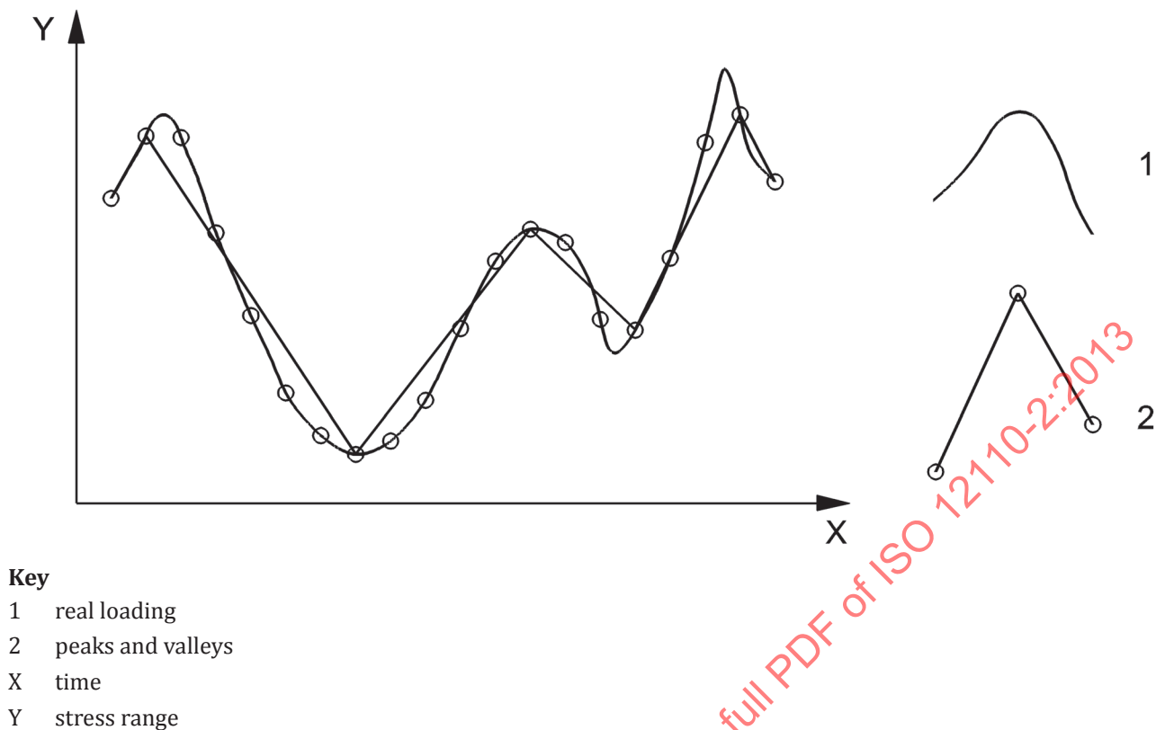
Figure A.2 — Loading signal after extracting peaks and valleys
