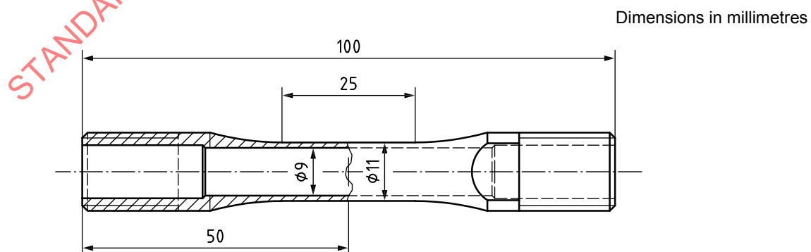
Figure 3 — Cylindrical smooth shank TMF tube (see Reference [3] in the Bibliography)
