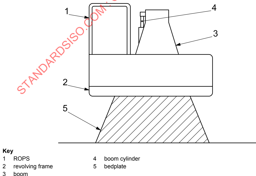
Figure 8 — Anchorage of revolving frame
