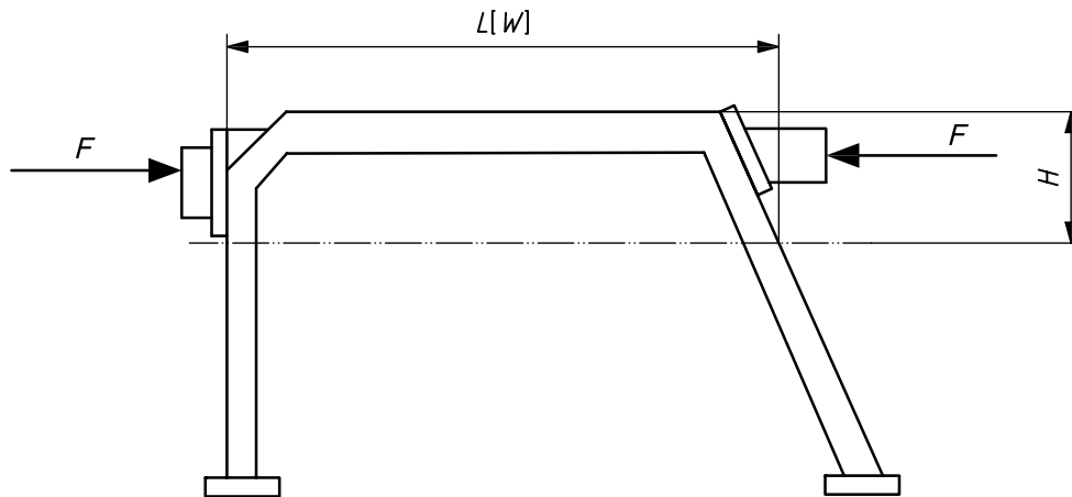
d) Example of shaped structural member showing load application
