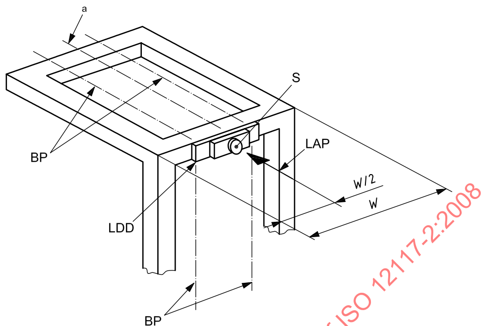
b) Longitudinal load distribution device in other cases
