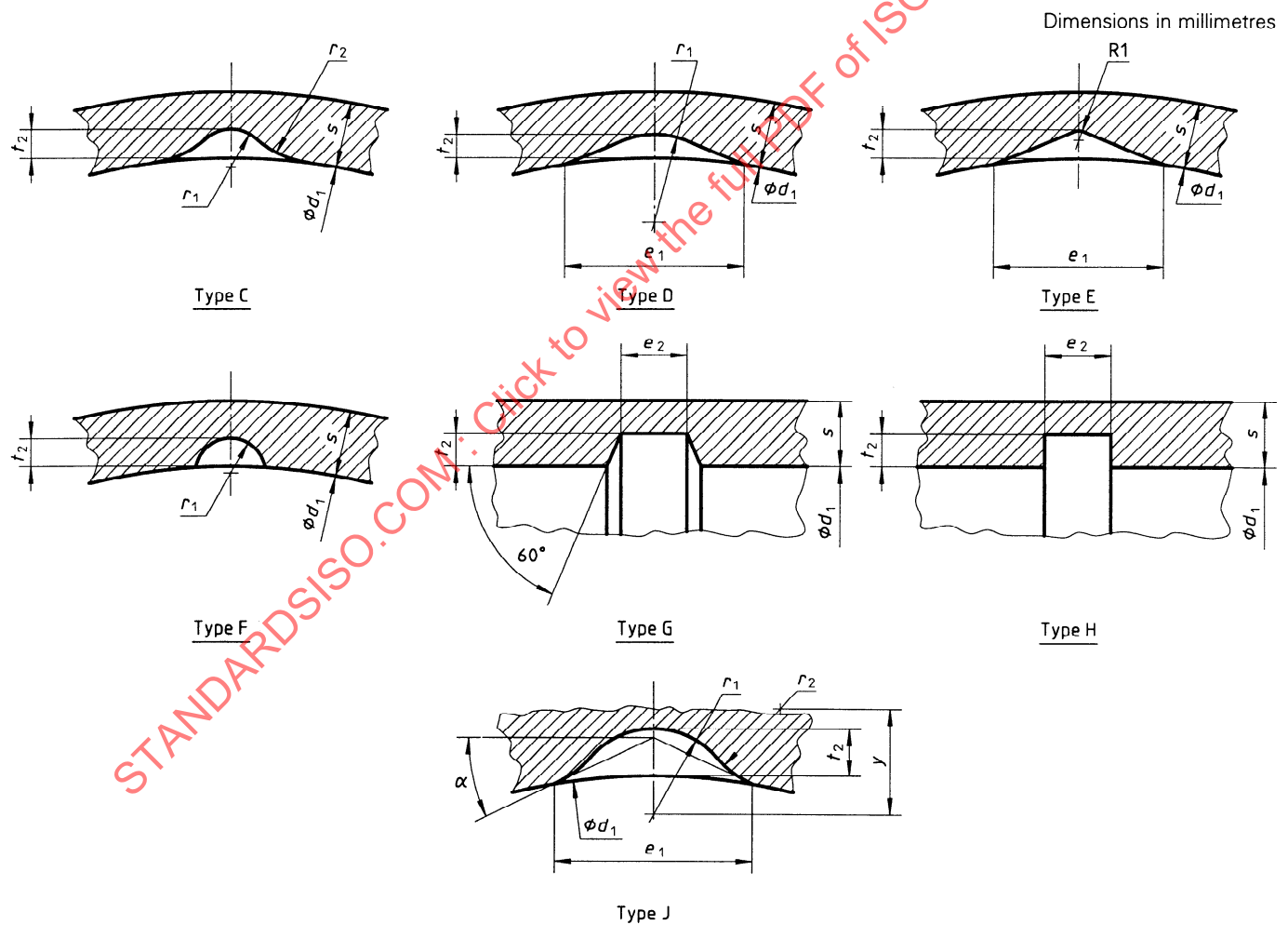
Figure 2 — Lubrication grooves
