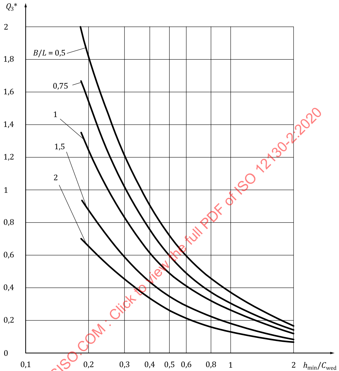
Figure 4 — Relative lubricant flow rate Q_3^* as a function of the relative bearing width, B/L , and the relative minimum lubricant film thickness, h_{\min}/C_{\text{wed}}
