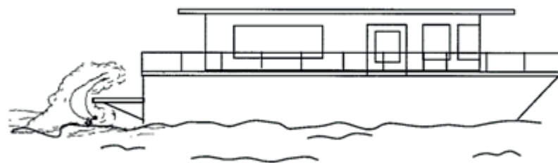
Figure A.2 — Accumulation of exhaust gases at the swim platform
