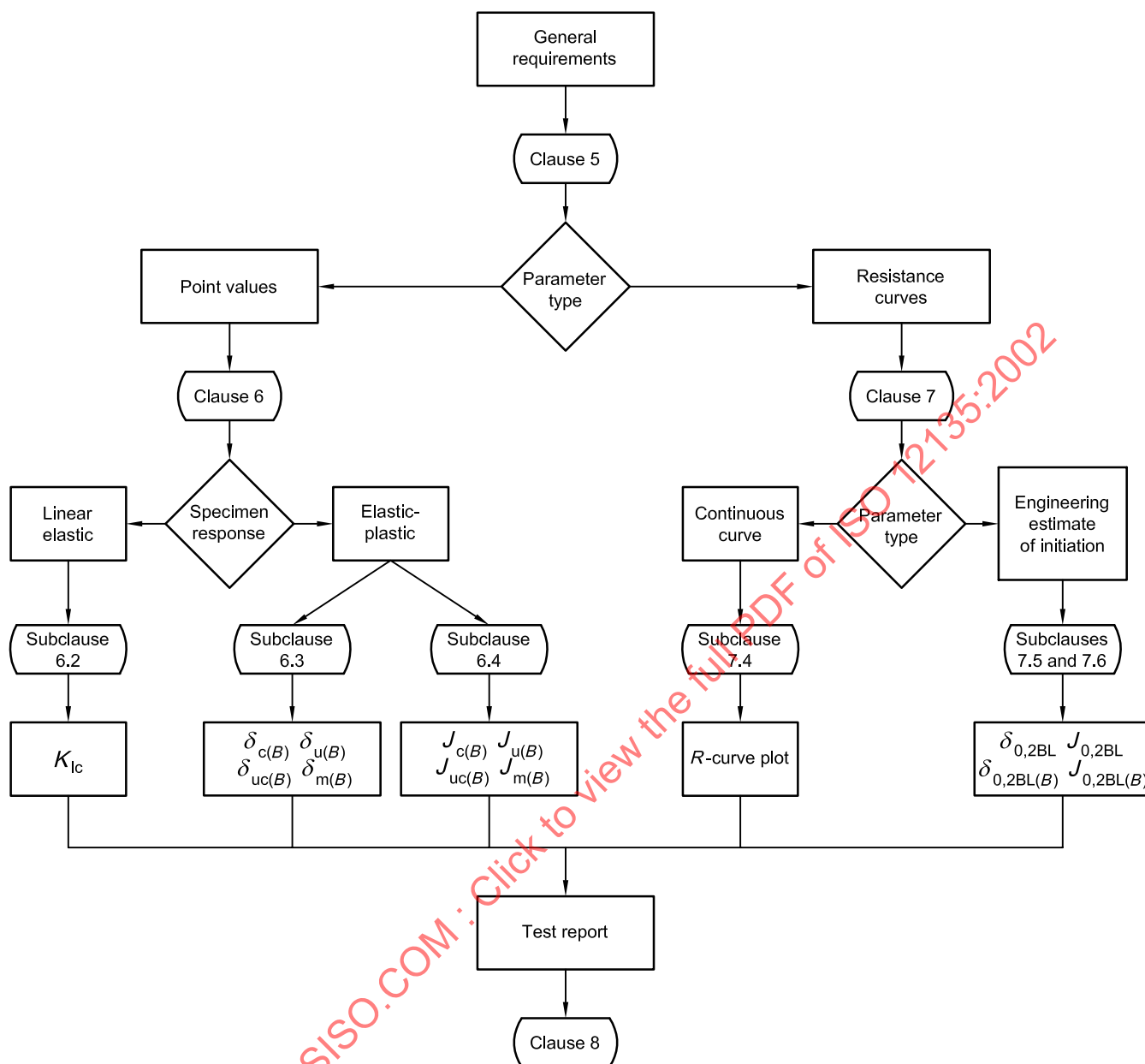
Figure 1 — General flowchart showing how to use the standard method of test
