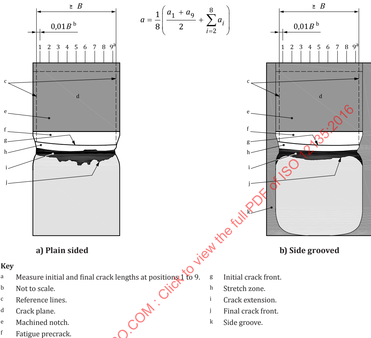
Figure 13 — Measurement of crack lengths on bend specimen
