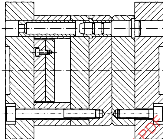
Figure 1 — Standard mould
