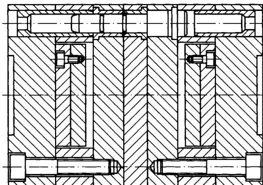
Figure 5 — Stack mould
