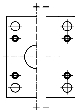
Figure 10 — Flush on all sides
