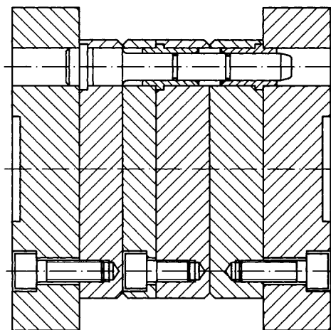
Figure 3 — Stripper plate mould
