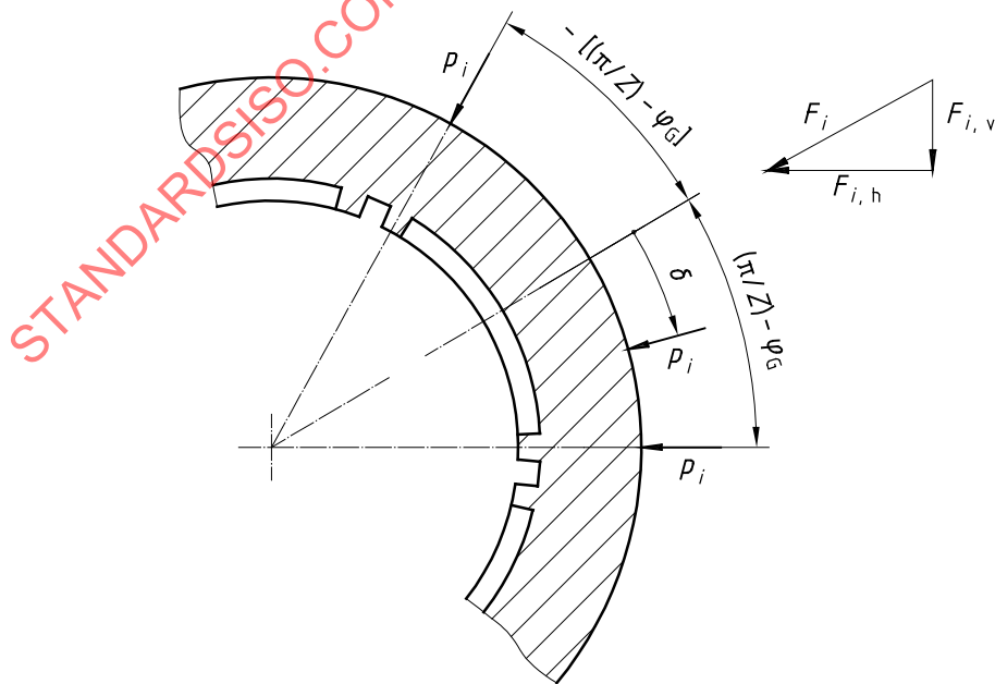
Figure A.5 — Application of load to one recess
