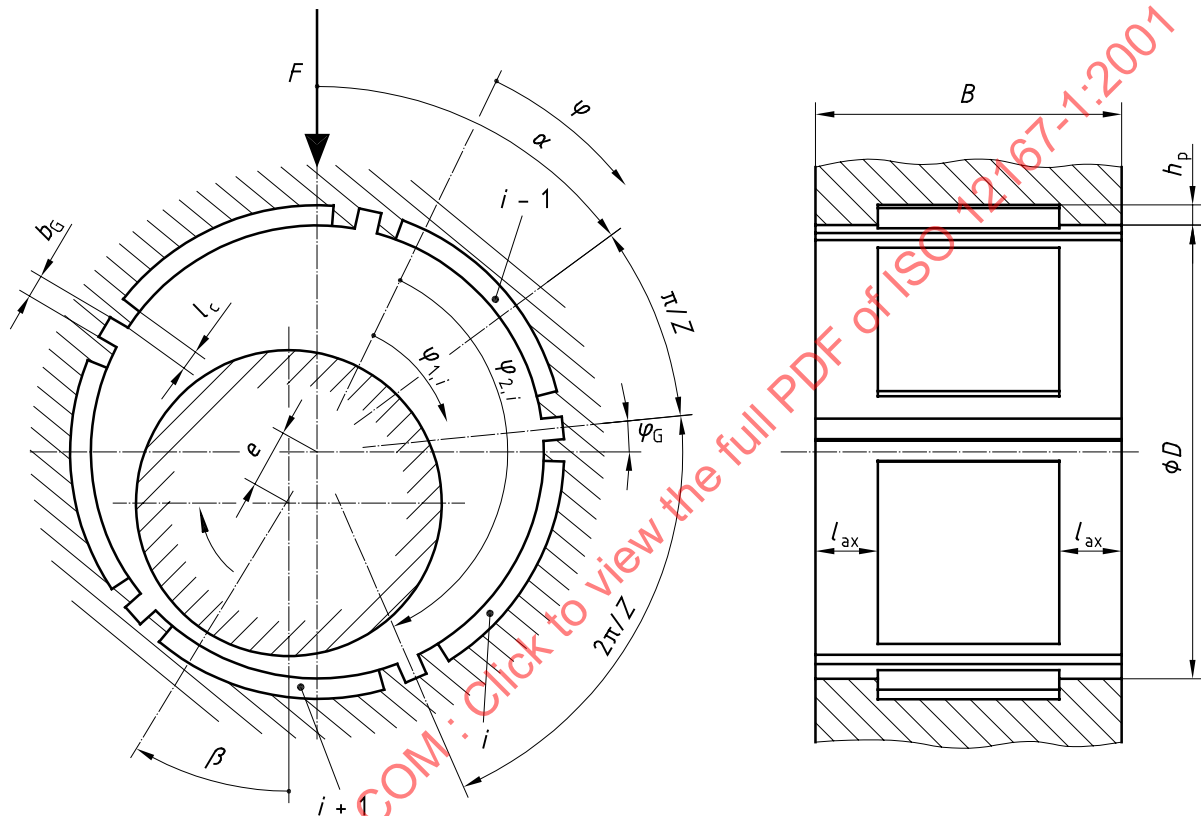
Figure A.3 — Bearing geometry
