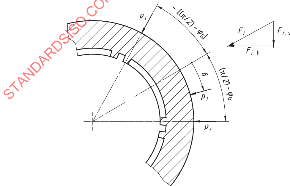
Figure A.5 — Application of load to one recess
