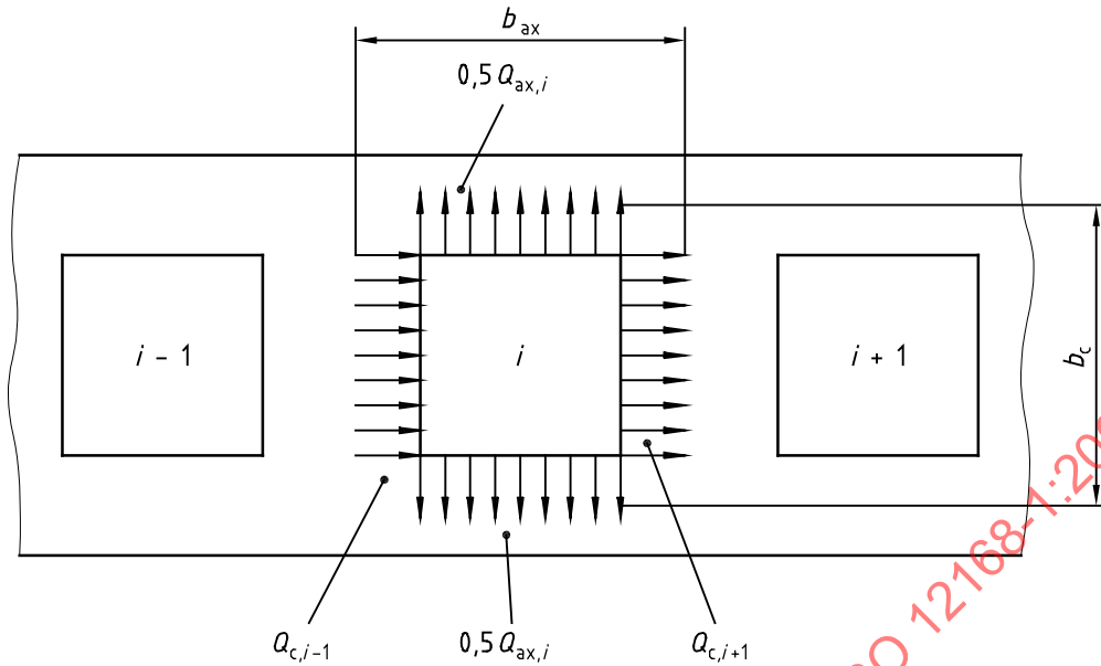
Figure A.4 — Volume flows for one recess
