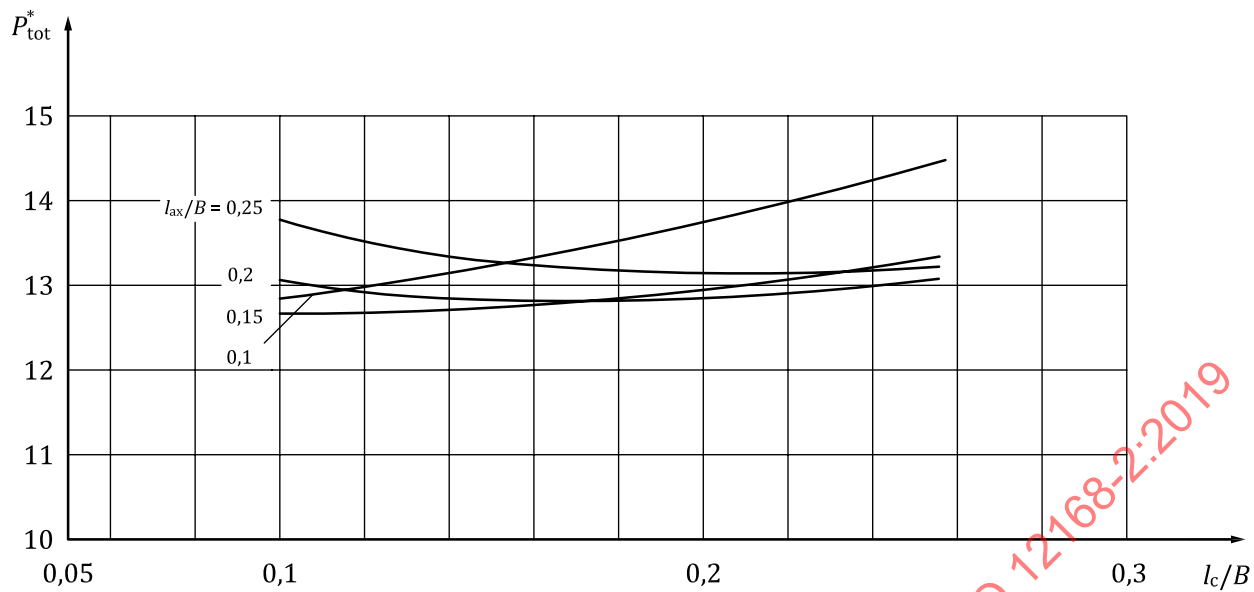
Figure 11 — Characteristic values of total power P_{\text{tot}}^* as a function of the relative land widths l_{\text{ax}}/B and l_c/B , \varepsilon = 0,4 ; B/D = 0,4 ; P^* = 2 ; Z = 10 ; \xi = 1 ; h_p = 40 \times C_R , with friction in the recesses
