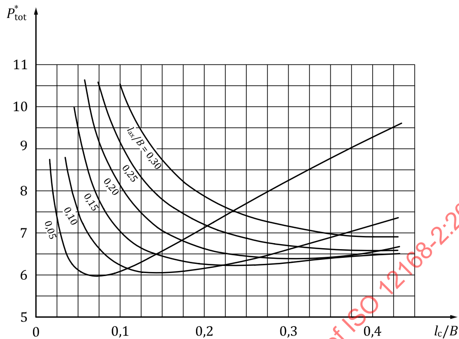
Figure 5 — Characteristic values of total power P_{\text{tot}}^* as a function of the relative land widths l_{\text{ax}}/B and l_{\text{c}}/B , B/D = 1 ; \varepsilon = 0,4 ; Z = 4 ; \xi = 1 ; P^* = 2 ; \alpha = 0 ; h_{\text{p}} = 40 \times C_{\text{R}} , without friction in the recesses
