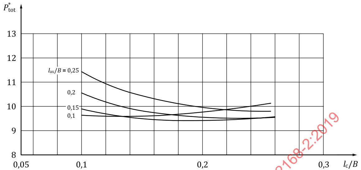
Figure 9 — Characteristic values of total power P_{\text{tot}}^* as a function of the relative land widths l_{\text{ax}}/B and l_c/B , \varepsilon = 0,4 ; B/D = 0,6 ; P^* = 2 ; Z = 6 ; \xi = 1 ; h_p = 40 \times C_R , with friction in the recesses
