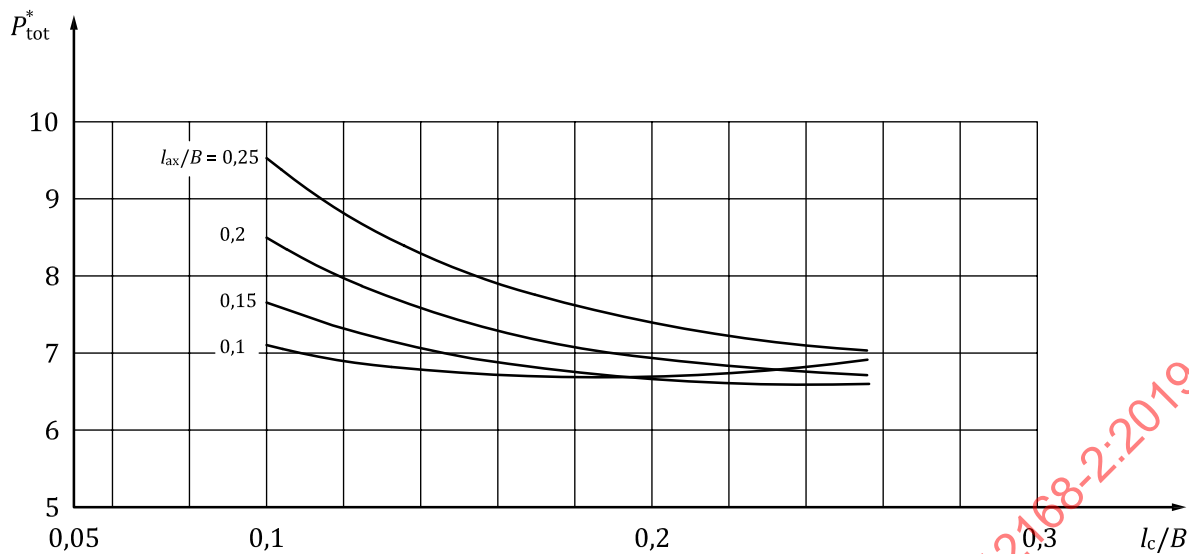
Figure 7 — Characteristic values of total power P_{tot}^* as a function of the relative land widths l_{ax}/B and l_c/B , \varepsilon = 0,4 ; B/D = 1 ; P^* = 2 ; Z = 4 ; \xi = 1 ; h_p = 40 \times C_R , with friction in the recesses
