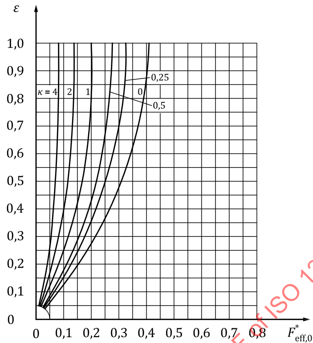
Figure 13 — Relative eccentricities \varepsilon as a function of the characteristic values of load-carrying capacity F_{\text{eff},0}^* for different resistance ratios \kappa and Z = 3 ; load directed to centre of the land [3]
