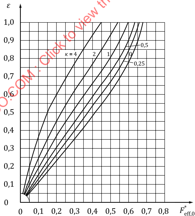
Figure 14 — Relative eccentricities \varepsilon as a function of the characteristic values of load-carrying capacity F_{\text{eff},0}^* for different resistance ratios \kappa and Z = 3 ; load directed to centre of the recess [3]
