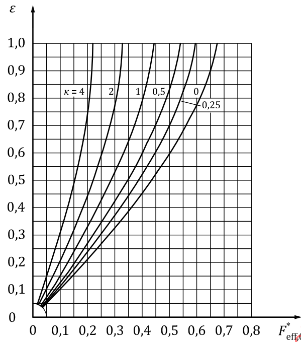
Figure 15 — Relative eccentricities \varepsilon as a function of the characteristic values of load-carrying capacity F_{\text{eff},0}^* for different resistance ratios \kappa and Z = 4 ; load directed to centre of the land [3]
