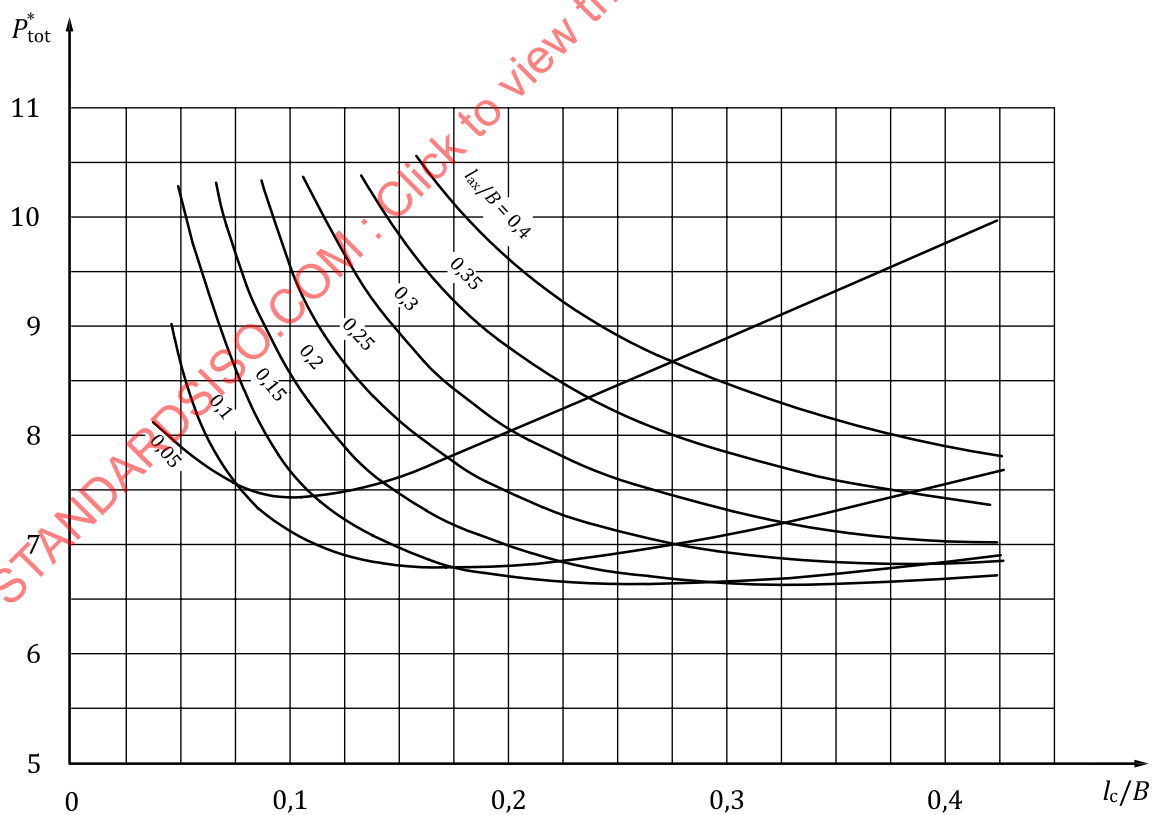
Figure 6 — Characteristic values of total power P_{\text{tot}}^* as a function of the relative land widths l_{\text{ax}}/B and l_{\text{c}}/B , B/D = 1 ; \varepsilon = 0,4 ; Z = 4 ; \xi = 1 ; P^* = 2 ; \alpha = 0 ; h_{\text{p}} = 40 \times C_{\text{R}} , with friction in the recesses
