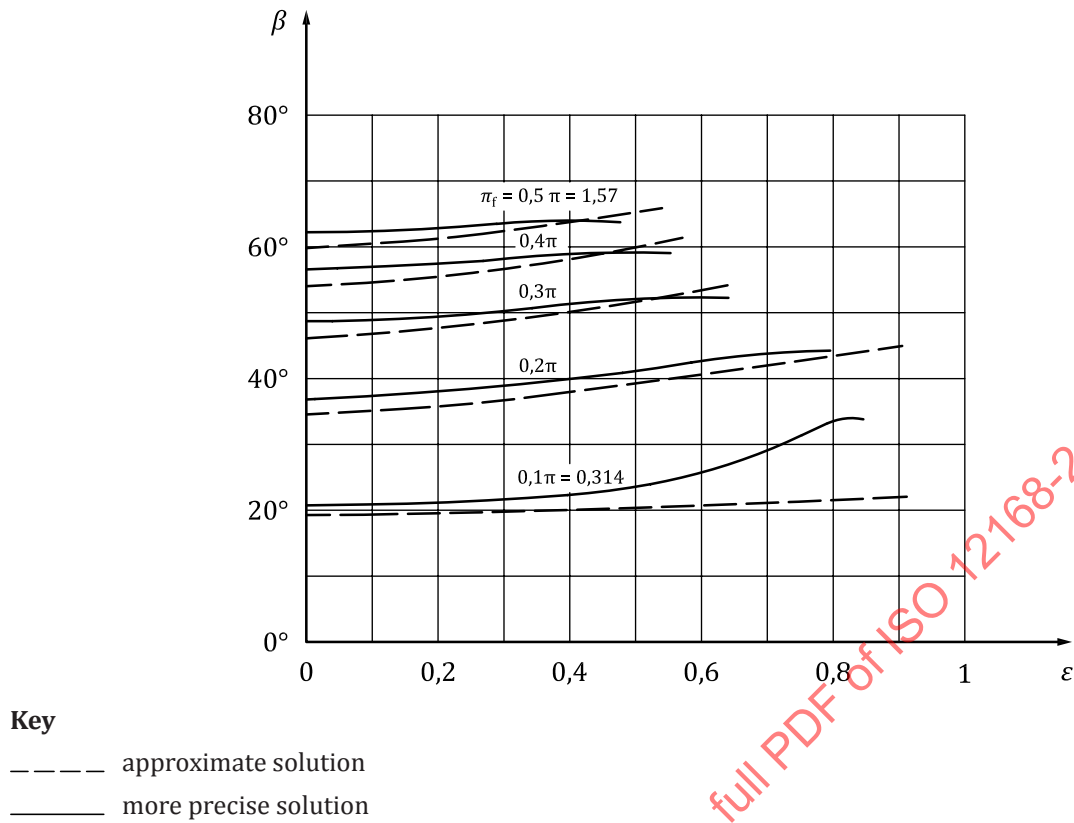
Figure 2 — Attitude angle \beta as a function of the relative eccentricity \varepsilon for different relative frictional pressures \pi_f and Z = 4 ; l_{ax}/B = 0,15 ; l_c/B = 0,25 ; B/D = 1 ; \xi = 1 ; \alpha = 0 [2]
