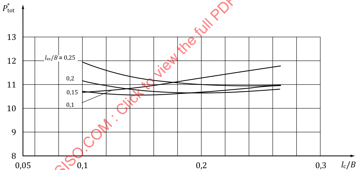
Figure 10 — Characteristic values of total power P_{\text{tot}}^* as a function of the relative land widths l_{\text{ax}}/B and l_c/B , \varepsilon = 0,4 ; B/D = 0,5 ; P^* = 2 ; Z = 8 ; \xi = 1 ; h_p = 40 \times C_R , with friction in the recesses
