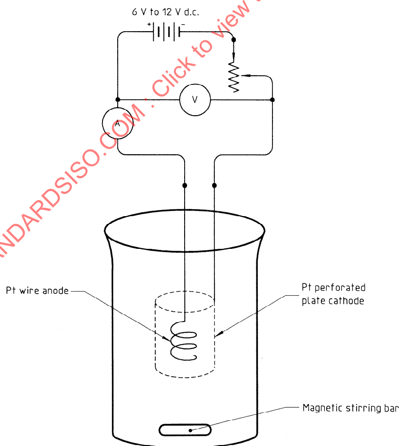
Figure 1 — Electrolytic deposition assembly
