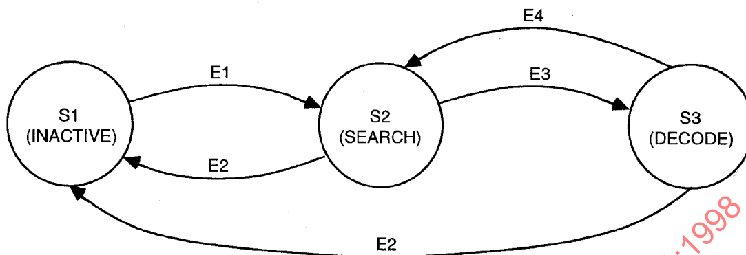
Figure 3-5: TC Channel Service State Diagram (Receiving End)
