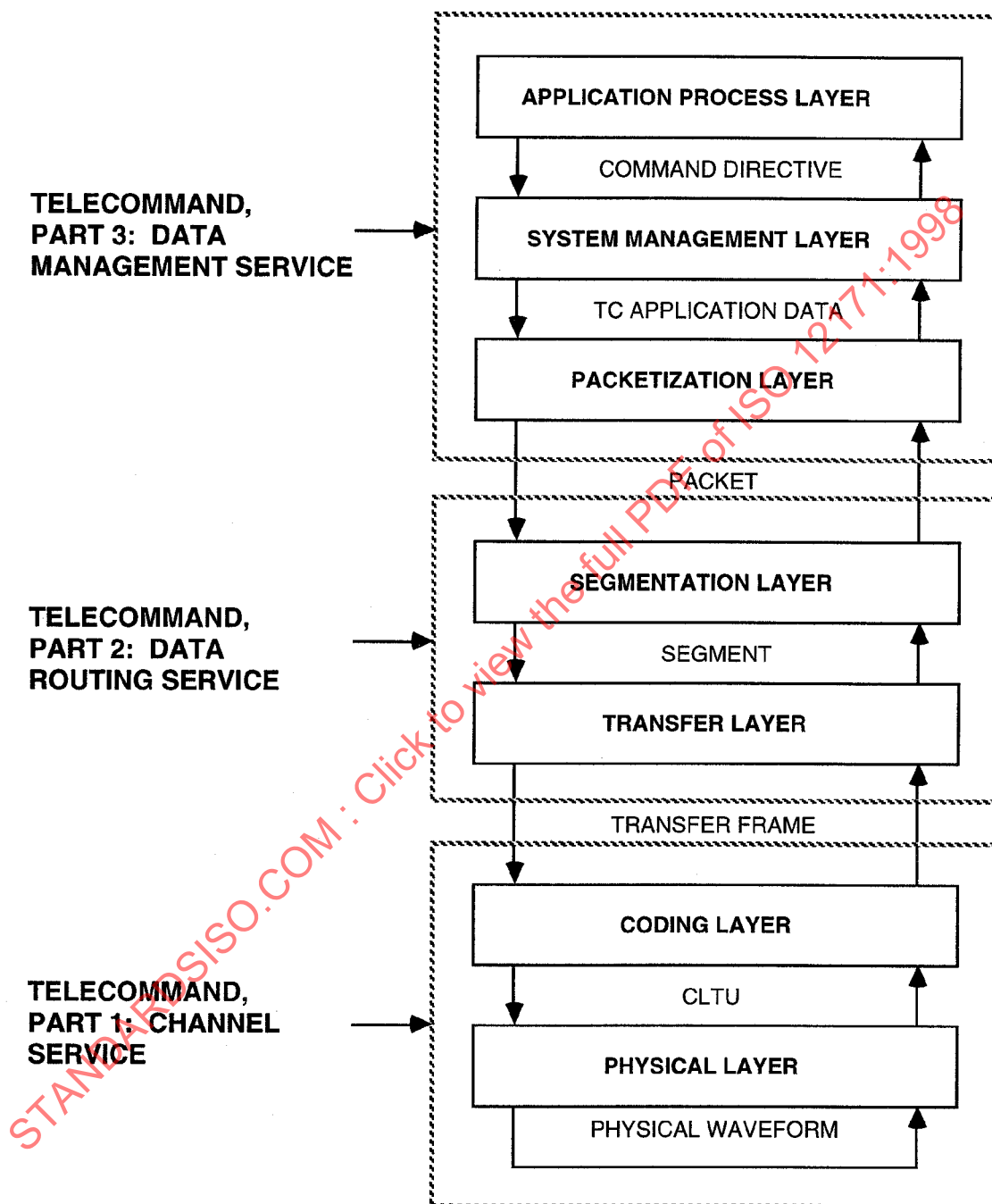
Figure 2-1: Telecommand System
