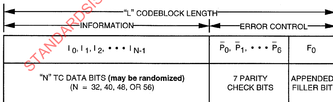
Figure 3-1: Telecommand Codeblock Format
