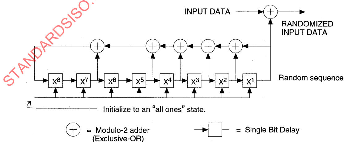
Figure 3-3: Bit Transition Generator Logic Diagram
