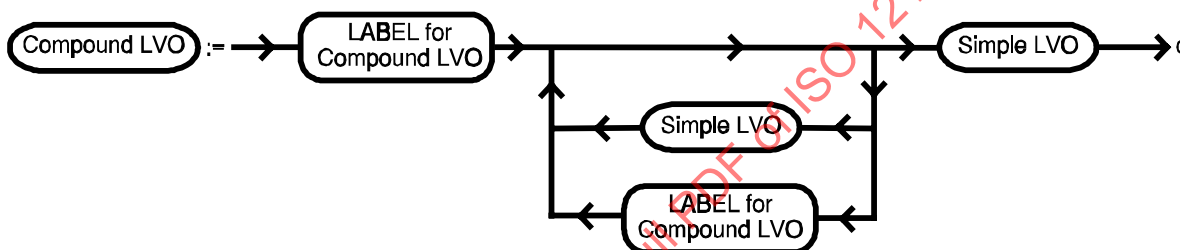
Figure 2-3: Structure Diagram of a Compound LVO
