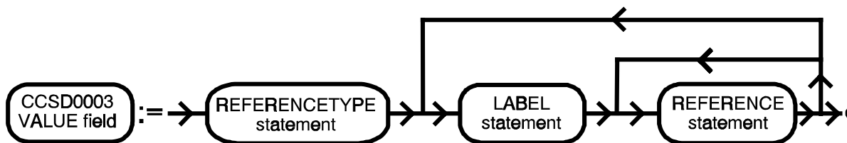
Figure 5-2: Structure Diagram of the PVL Statements within an LVO with ADID = CCSD0003
