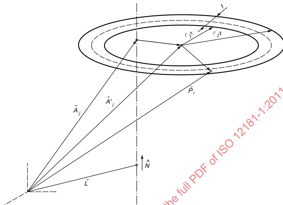
Figure A.1 — Roundness tolerance zone of a nominal integral feature
