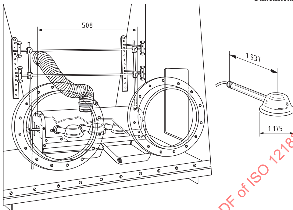
Figure 1 — Sample evaporation system
