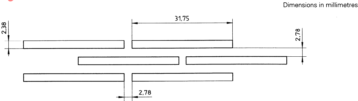
Figure 5 — Location of dampers
