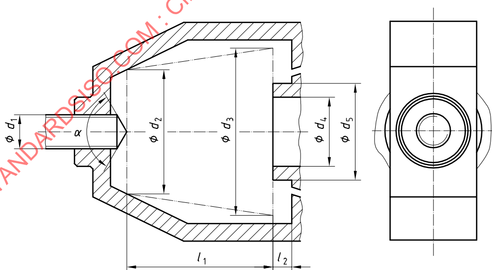
Figure 3 — Yoke
