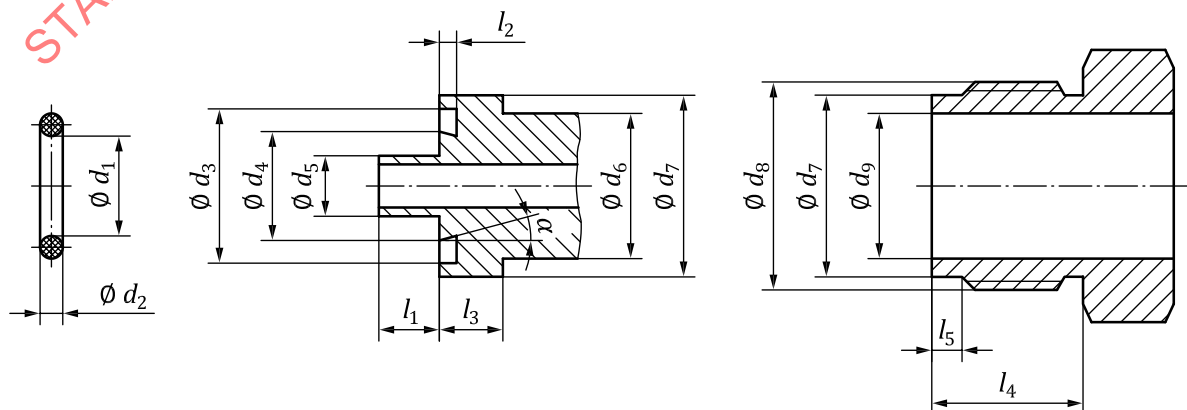
Figure 11 — 300 bar filling connector — Components
