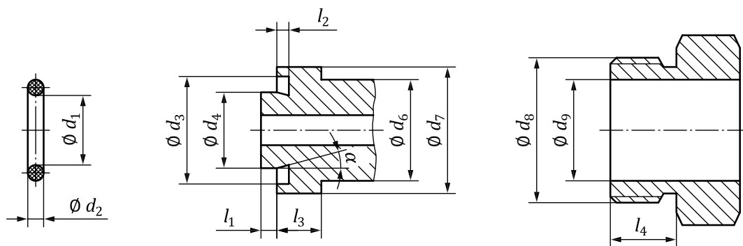
Figure 8 — 232 bar gas withdrawal connector — Components
