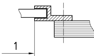
d) Glued or elastomer in a frame
