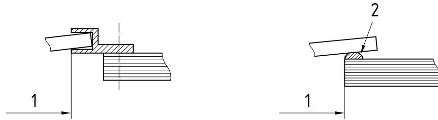
a) Sliding in a frame or a rabbet
