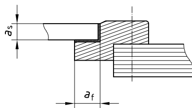
Figure D.5 — Glued joint dimensions sketch
