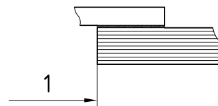
c) Bolted with counter frame and jointing compound
