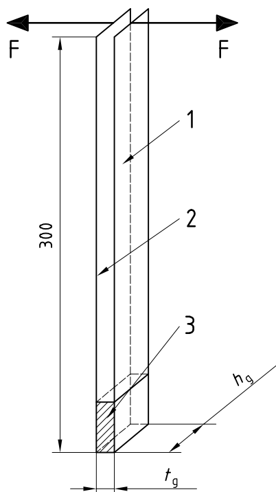
Figure D.6 — Arrangement for the separation test
