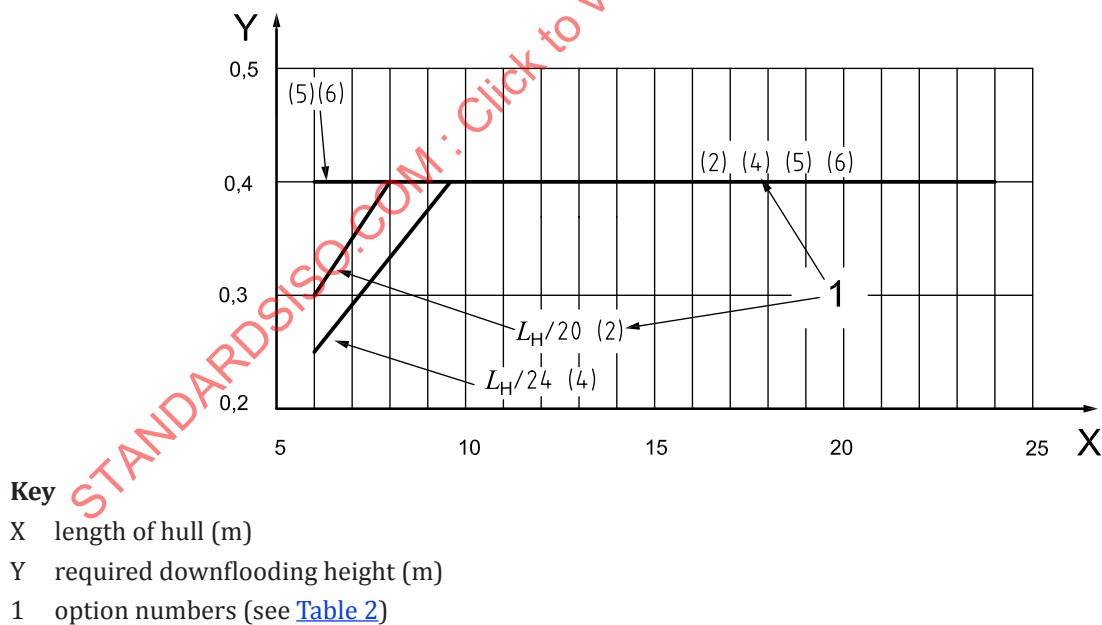
Figure 4 — Required downflooding height — design category D
