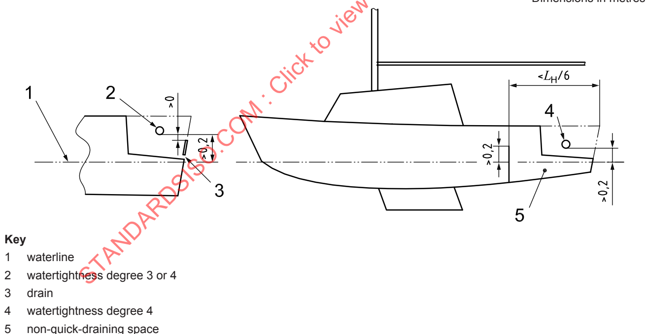
Figure 1 — Openings in outboard engine wells
