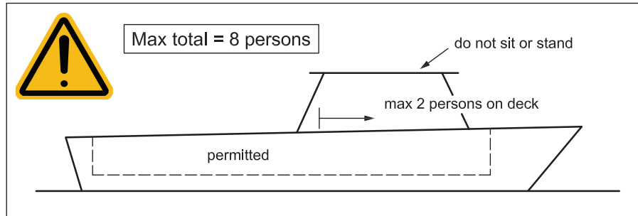
Figure Amd.1-2 — Example of crew area and access limitation label for control position (using ISO 7010 – W001 “General warning”)
