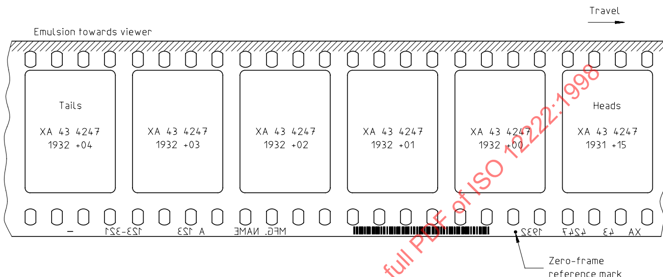
Figure 7 — Alignment of zero-frame reference mark on 35 mm film
