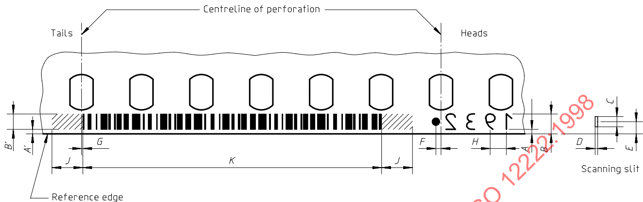
Figure 8 — Key number position and dimensions on 65 mm film
