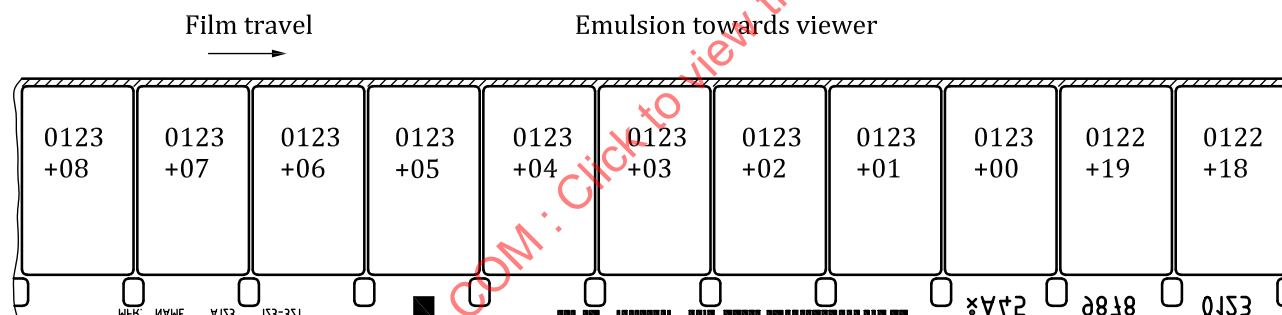
Figure 5 — Alignment of zero-frame reference mark on 16 mm film
