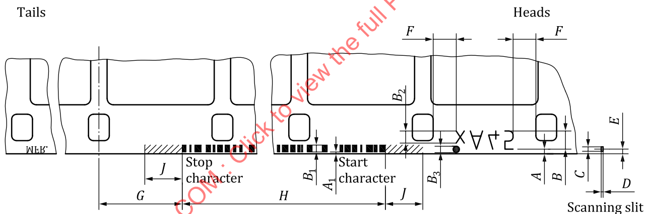
Figure 4 — Key number position and dimensions on 16 mm film
