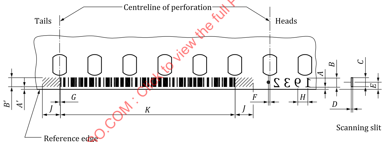
Figure 8 — Key number position and dimensions on 65 mm film, format A and format B
